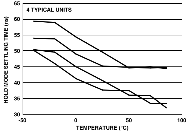
FIGURE 10. HOLD MODE SETTTLING vs TEMPERATURE
